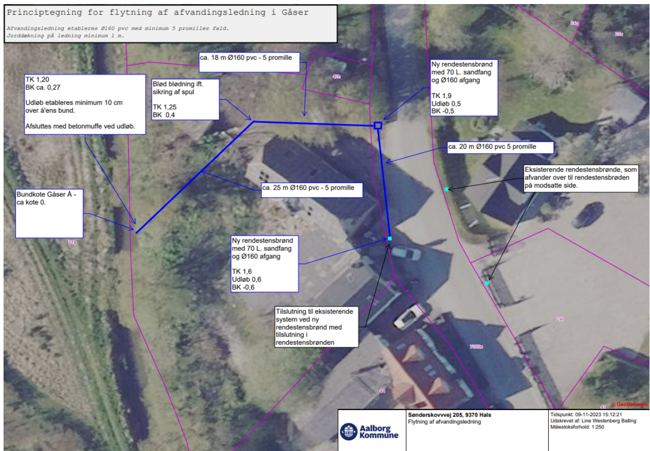
Figur 1: Situationsplan over regnvandssystem.
